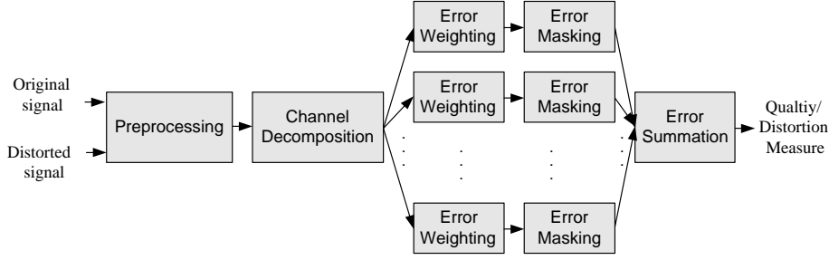
Fig. 1. Error sensitivity based image quality measurement.
