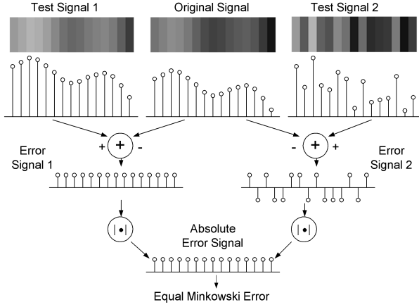
Fig. 2. Minkowski error pooling.
