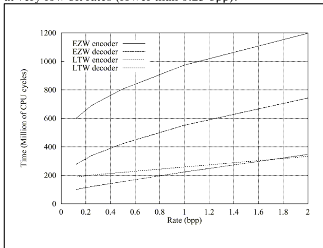
Fig. 2. Execution time comparison (EZW and LTW)
