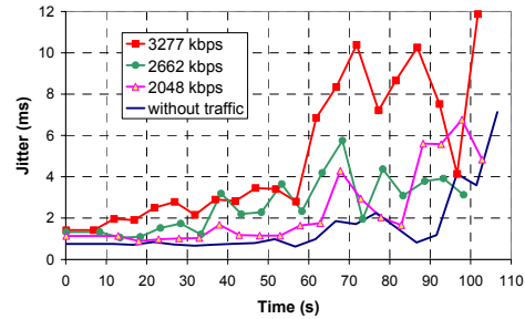
Figure 6. Jitter comparison at different background traffic loads (MPEG-4 video codec).
