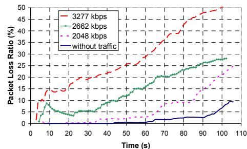
Figure 7. PLR evolution using MPEG-4 codec with different background traffic loads.
