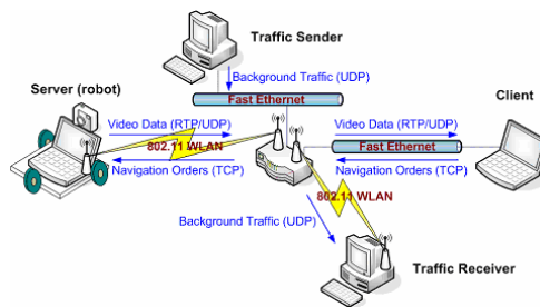
Figure 1. Overview of the telerobotic experimental platform.
