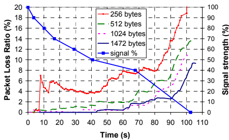
Figure 5. Signal strength and PLR for different packet sizes.
