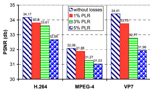
Figure 3. R/D performance of codecs under packet losses.
