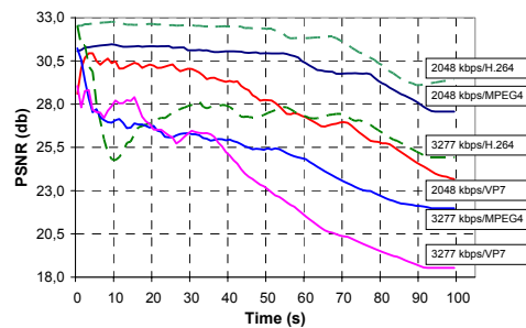
Figure 9. Quality of reconstructed video with different codecs and traffic loads.
