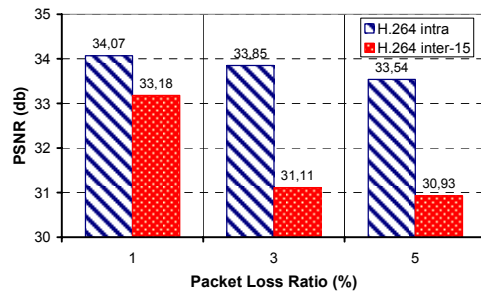
Figure 4. Resilience of intra and inter compression modes.
