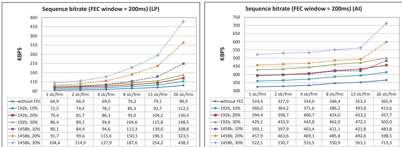
Fig. 3 Bitrate (kbps) without FEC protection and with FEC protection for different symbol sizes, different protection windows and different number of slices per frame (including RTP and fragmentation headers). Left: LP mode. Right: AI mode.
