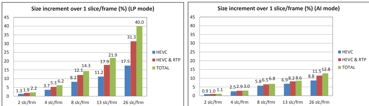
Fig. 2 Percentage of bitrate increase (without FEC protection) for different number of slices per frame. Left: LP mode. Right: AI mode. ( HEVC raw bitstream // HEVC + RTP header // HEVC + RTP header + fragmentation header )
