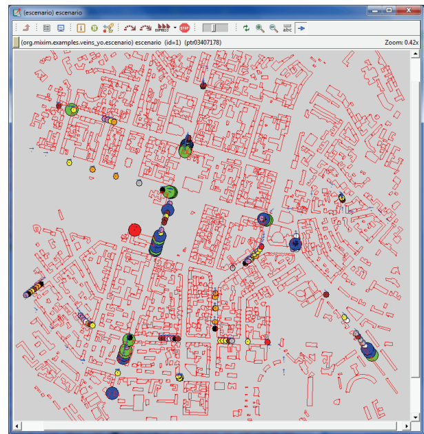
Figure 6. City of Kiev in OMNeT++/Veins. Red polygons represent obstacles (buildings). Blue arrows denote vehicles. Big circles surround vehicles transmitting or receiving video. Small circles surround vehicles receiving other kind of data.
